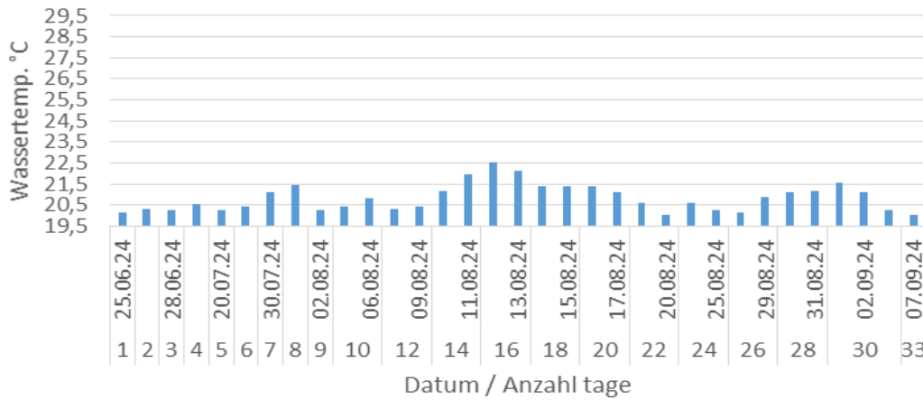
Wassertemperatur Elz _Brettenbach 2024 - IG-Elz_13 (Tage \geq 20^\circ\text{C} )
