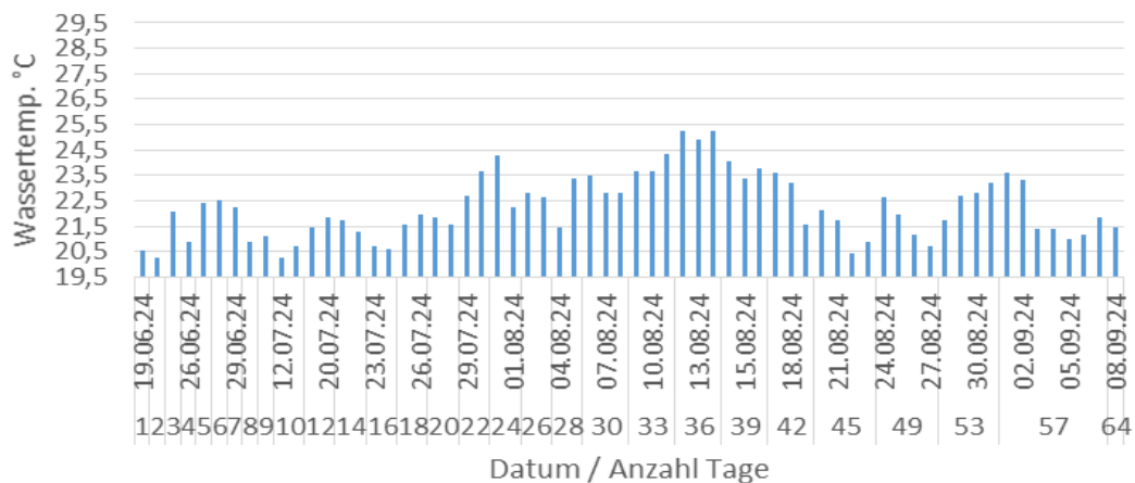
Wassertemperatur Brettenbach 2024 - IG-Elz_4 (Tage \geq 20^\circ\text{C} )
