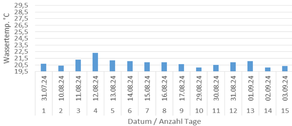
Wassertemperatur Elz 2024 - IG-Elz_2 (Tage \geq 20^\circ\text{C} )
