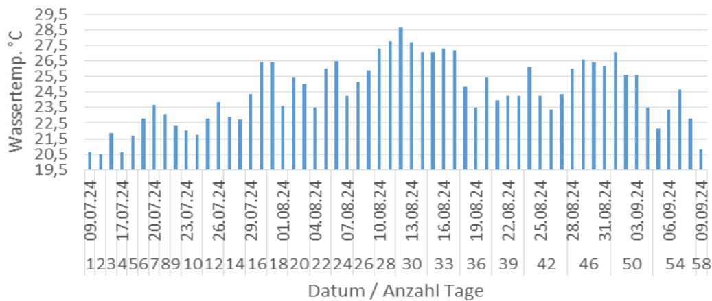
Wassertemperatur Elz 2024 - IG-Elz_3 (Tage \geq 20^\circ\text{C} )
