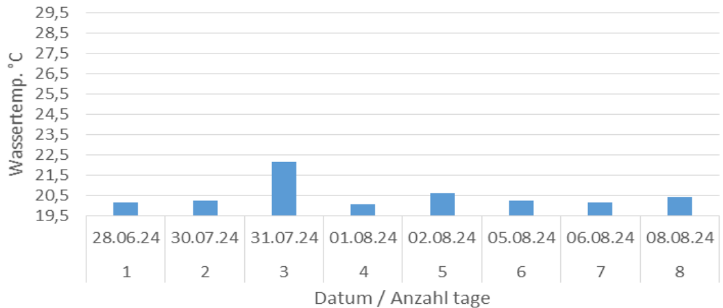
Wassertemperatur Elz 2024_Kollnau - IG-Elz_9 (Tage \geq 20^\circ\text{C} )
