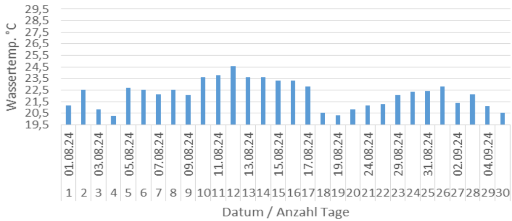
Wassertemperatur Elz 2024 - IG-Elz_6 (Tage \geq 20^\circ\text{C} )
