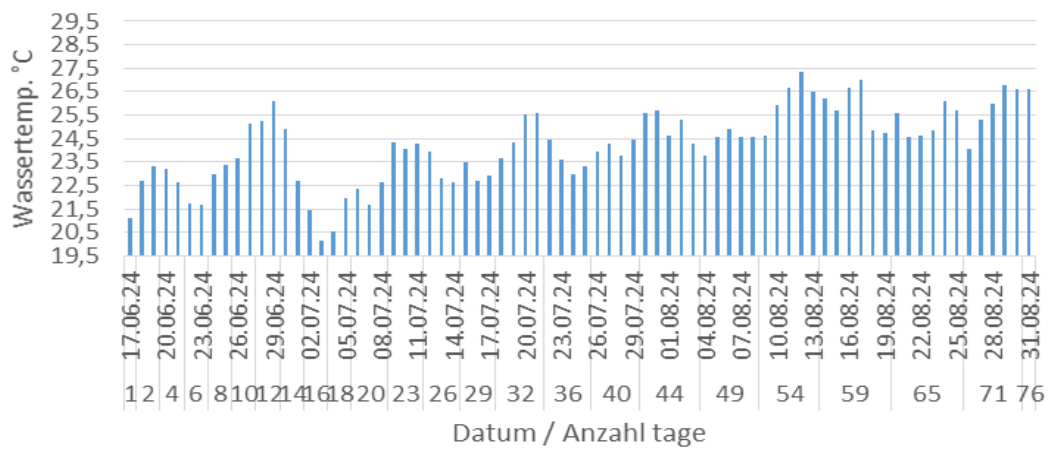
Wassertemperatur Elz 2024 - IG-Elz_7 (Tage \geq 20^\circ\text{C} )
