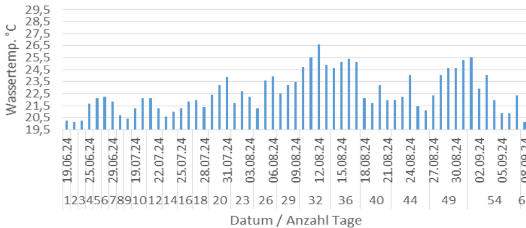
Wassertemperatur Elz 2024 - IG-Elz_15 (Tage \geq 20^\circ\text{C} )
