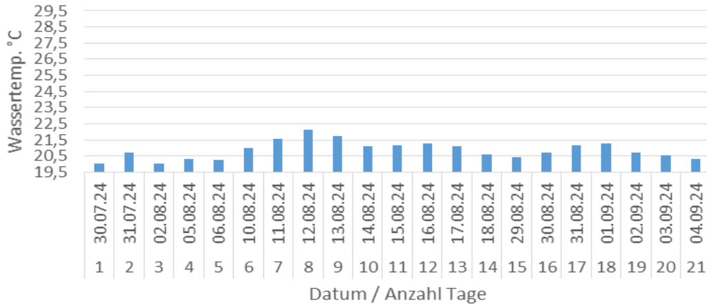
Wassertemperatur Elz 2024 - IG-Elz_10 (Tage \geq 20^\circ\text{C} )
